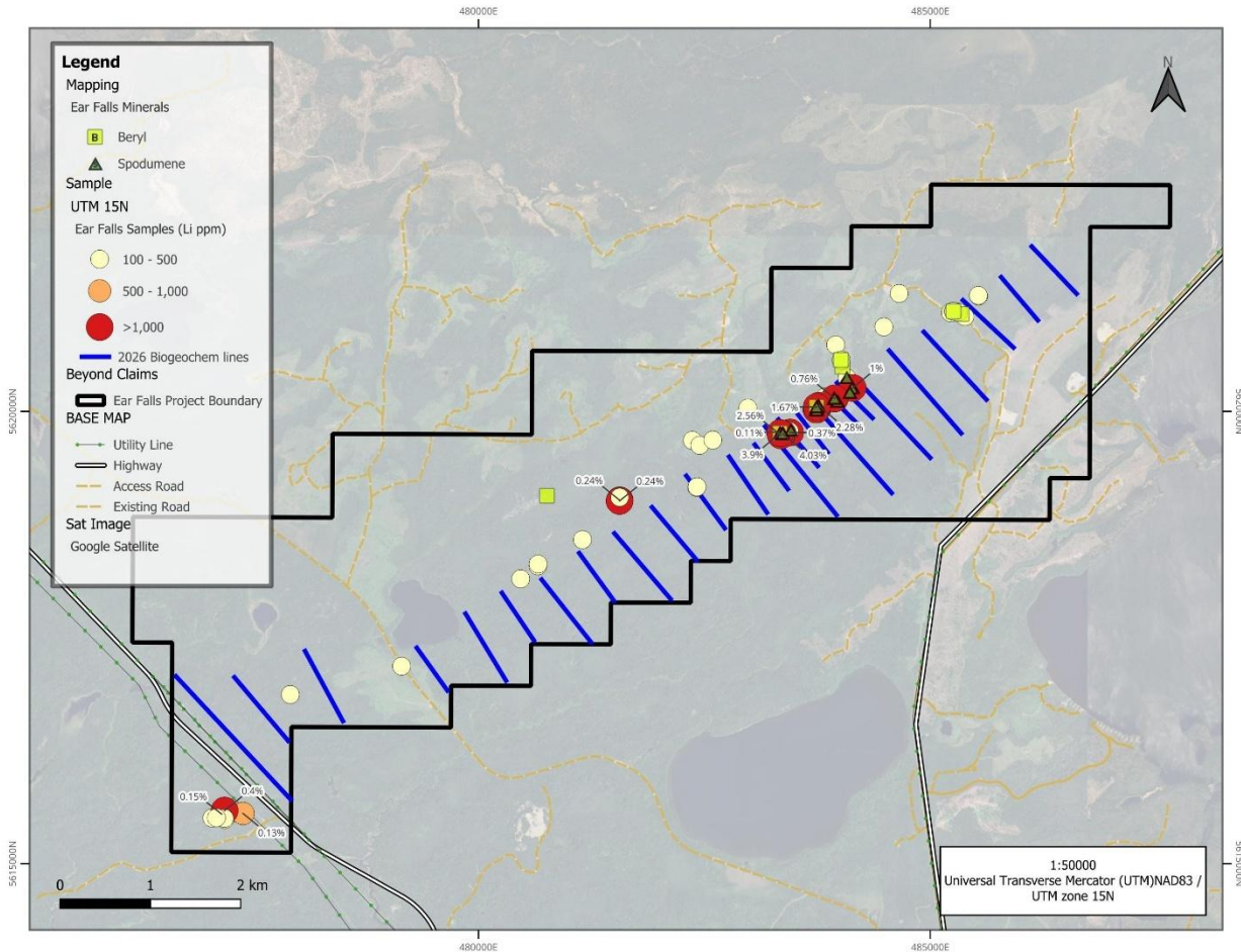
Figure 2. Ear Falls 2026 Biogeochemical Survey Lines Map
